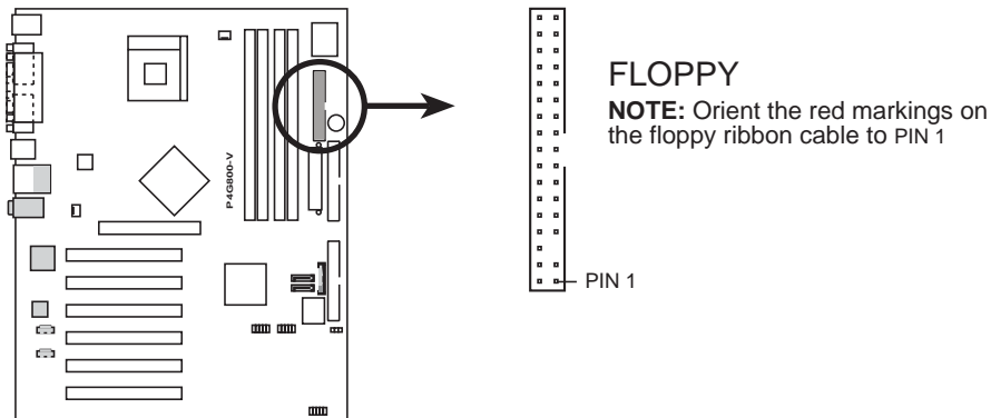
P4G800-V Floppy Disk Drive Connector
