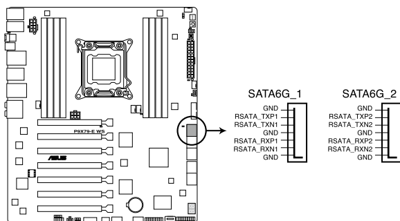
P9X79-E WS Intel® SATA 6.0 Gb/s connectors
