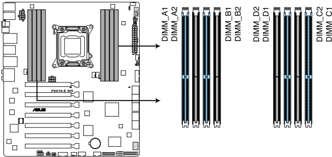
P9X79-E WS 240-pin DDR3 DIMM socket
