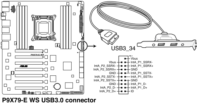
P9X79-E WS USB3.0 connector
