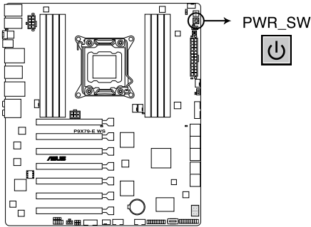
P9X79-E WS Power on button
