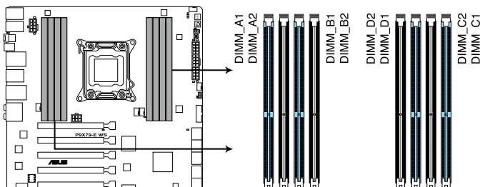
P9X79-E WS 240-pin DDR3 DIMM socket
