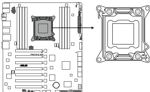
P9X79-E WS CPU LGA2011
