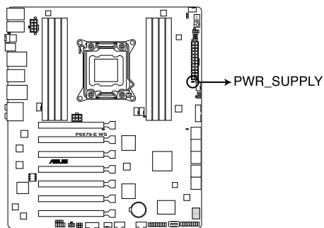
P9X79-E WS PWR_SUPPLY LED
