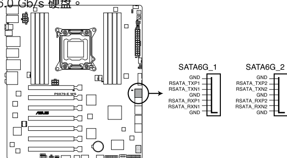
P9X79-E WS Intel® SATA 6.0 Gb/s connectors
