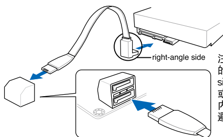
P9X79-E WS Intel® SATA 6.0 Gb/s connectors
