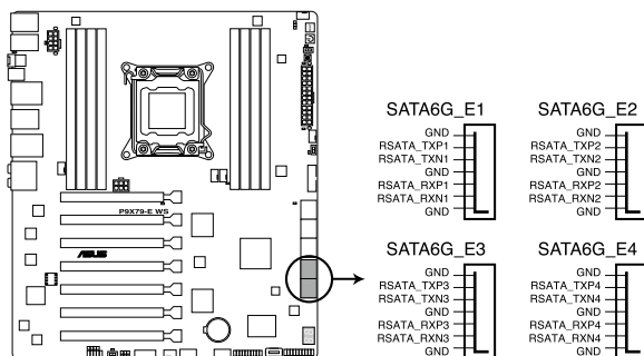
P9X79-E WS Marvell® SATA 6.0 Gb/s connectors
