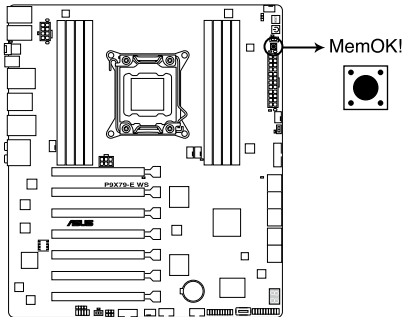
P9X79-E WS MemOK! button
