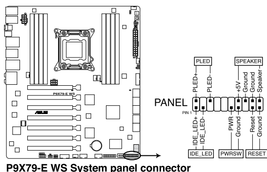
P9X79-E WS System panel connector
