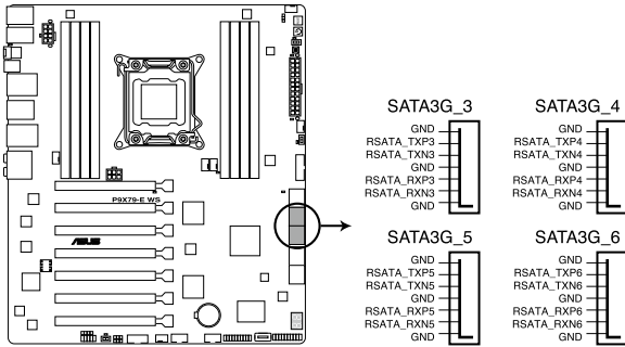
P9X79-E WS Intel® SATA 3.0 Gb/s connectors
