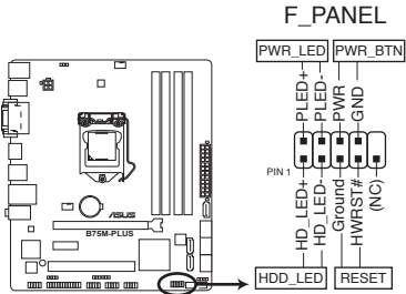
B75M-PLUS System panel connector
