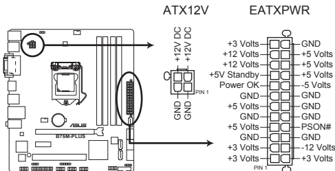
B75M-PLUS ATX power connectors
