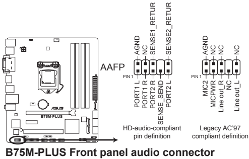
B75M-PLUS Front panel audio connector
