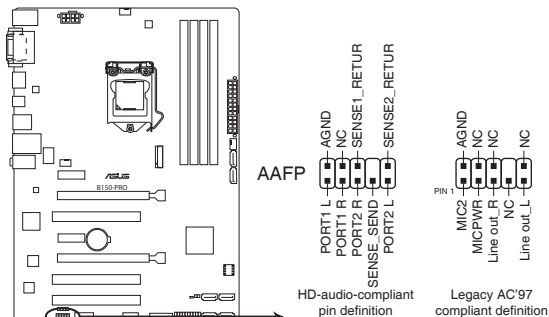
B150-PRO Front panel audio connector
