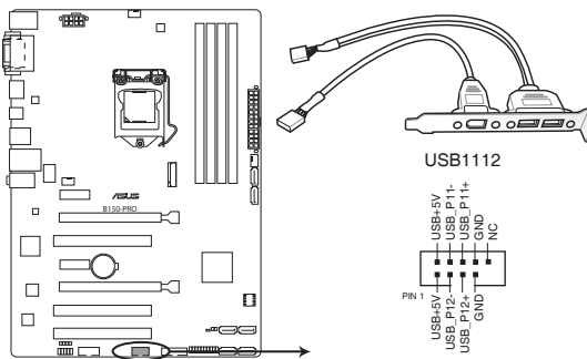
B150-PRO USB2.0 connector
