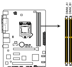
H81M-C 240-pin DDR3 DIMM sockets
